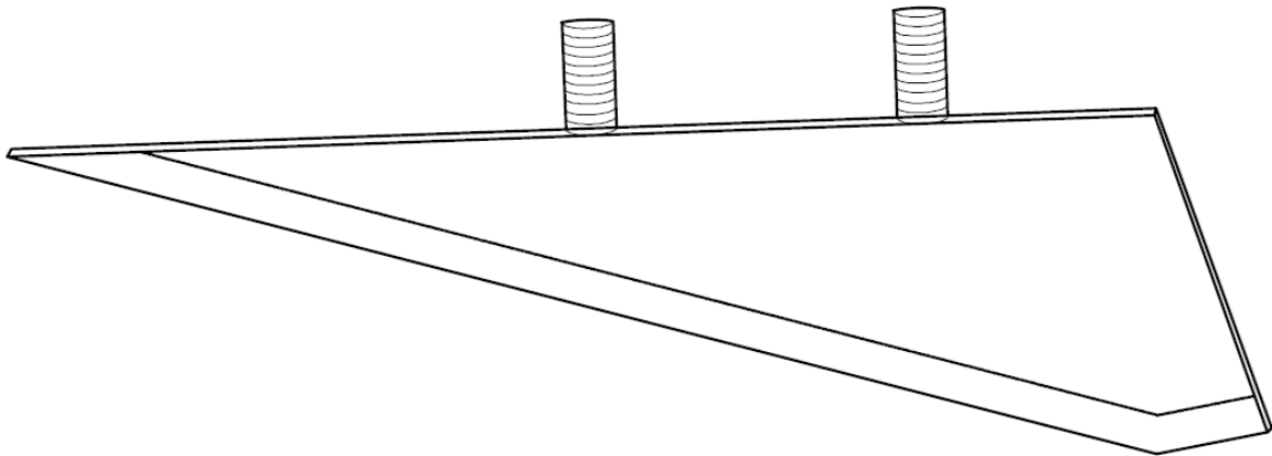
D800-324—LOCKWOOD SHOE ASSEMBLY
